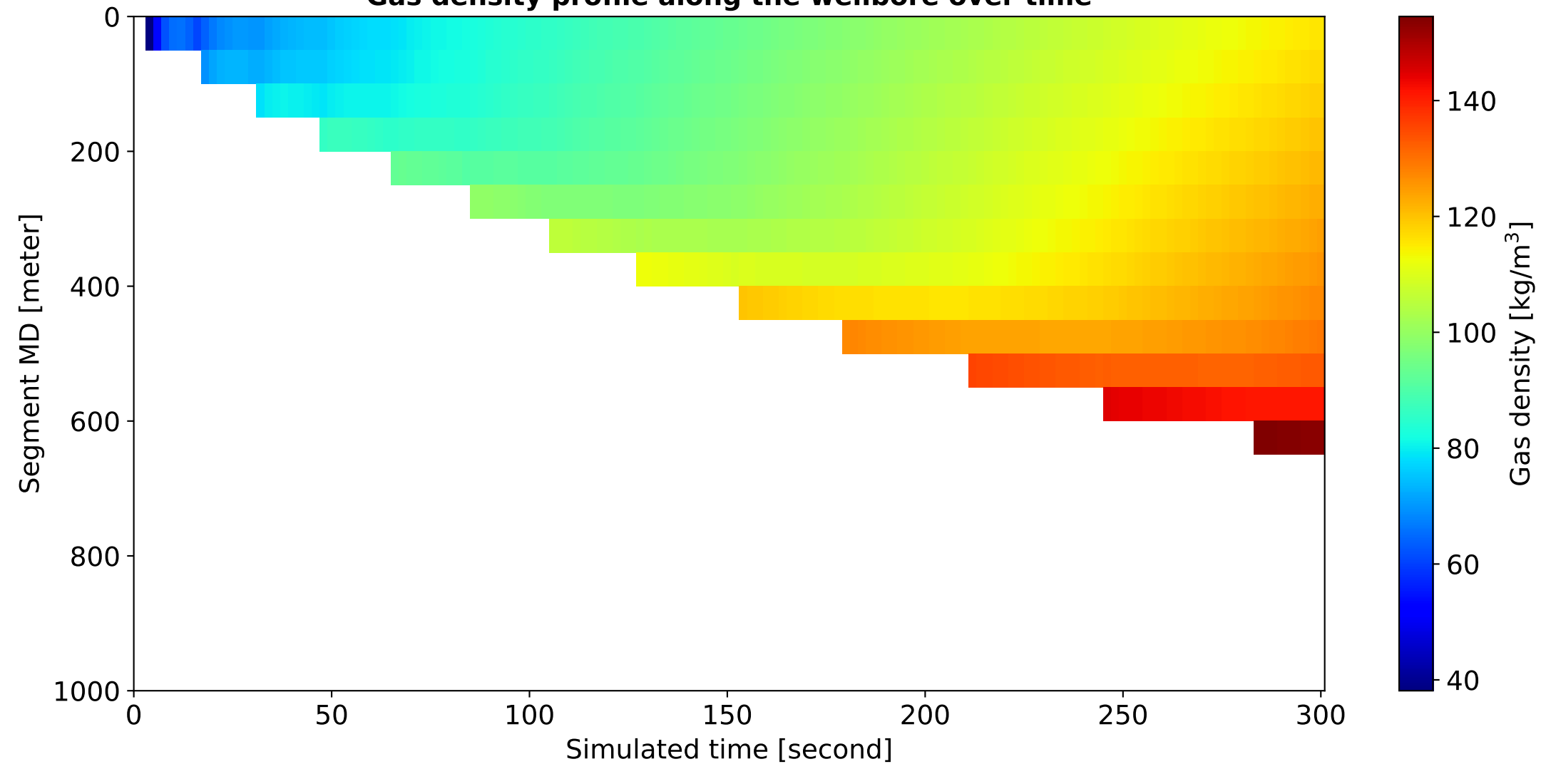
Gas density profile along the wellbore over time
